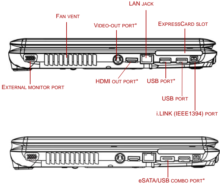
Figure 2-2 The left side of the computer
